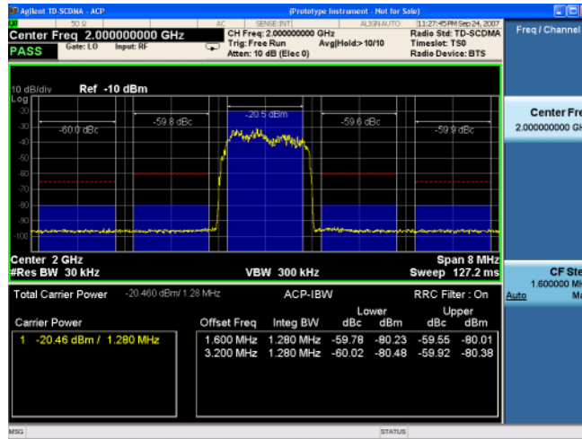
Figure 2-6 ACP - Bar Graph View (Default)
