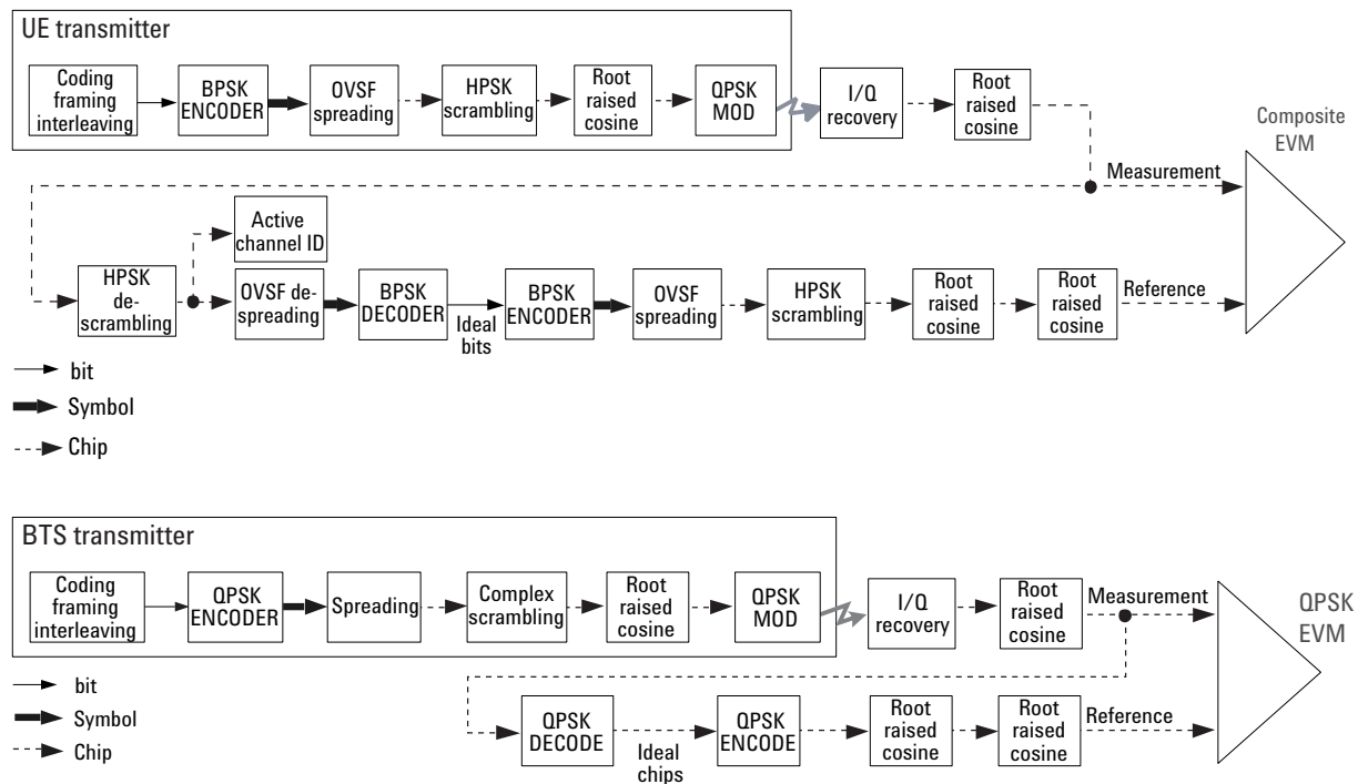
Figure 4-16 Process to Calculate Composite EVM for TD-SCDMA Signal
