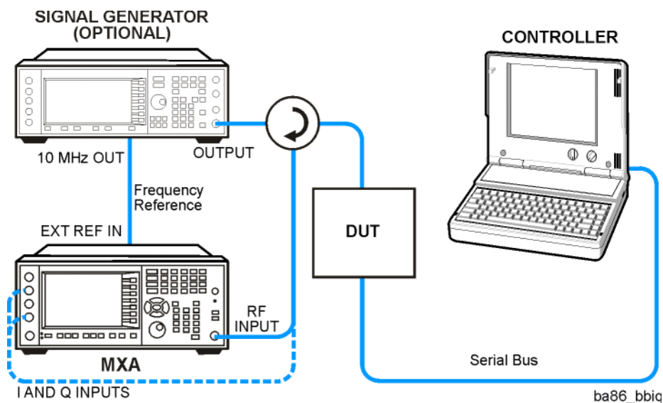
Code Domain Power Measurement System—Baseband
