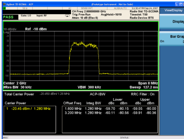
Figure 2-7 ACP - Bar Graph Off
