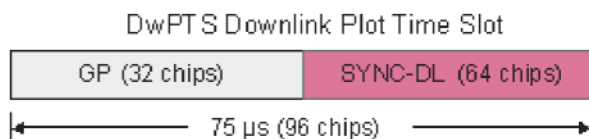
Figure 4-4 Downlink Pilot Time Slot
