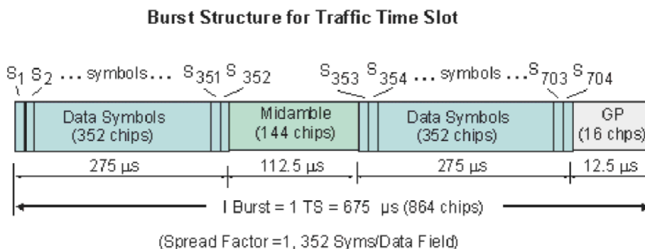
Figure 4-3 Burst Structure for Traffic Time Slot
