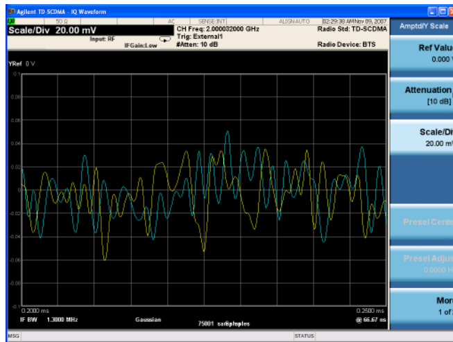
Figure 2-41 Monitor Spectrum Measurement - I/Q Waveform view
