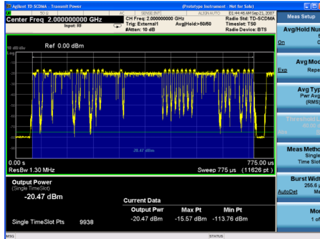
Figure 2-2 Transmit Power - Single Timeslot
