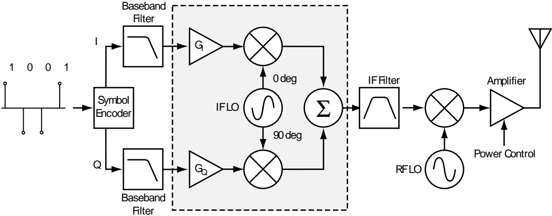
Figure 4-9 I/Q Modulator a source of Impairments
