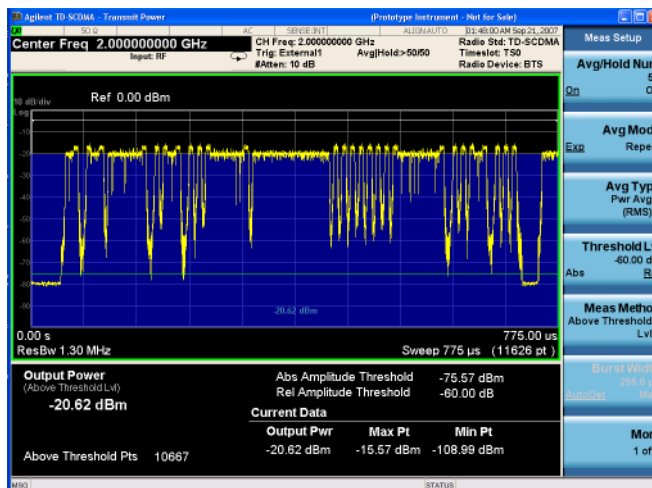
Figure 2-4 Transmit Power - Above Threshold Lvl
