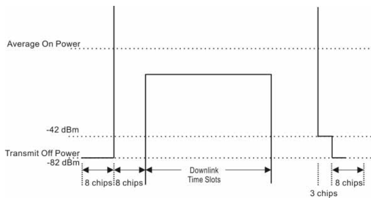
Figure 4-6 Power vs Time Measurement BTS Mask
