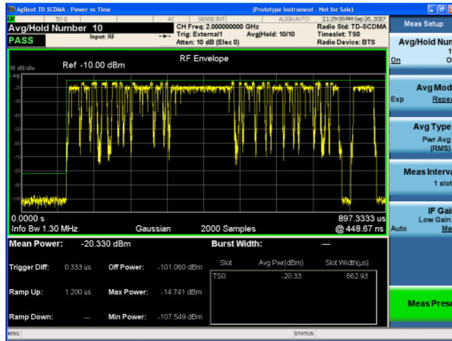
Figure 2-10 Power vs Time - Single-Slot View (Default)
