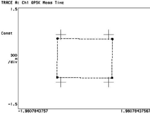
Figure 4-10 I/Q Gain Imbalance
