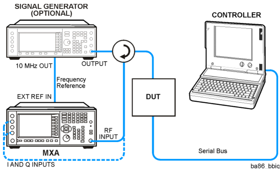
Code Domain Power Measurement System—Baseband
