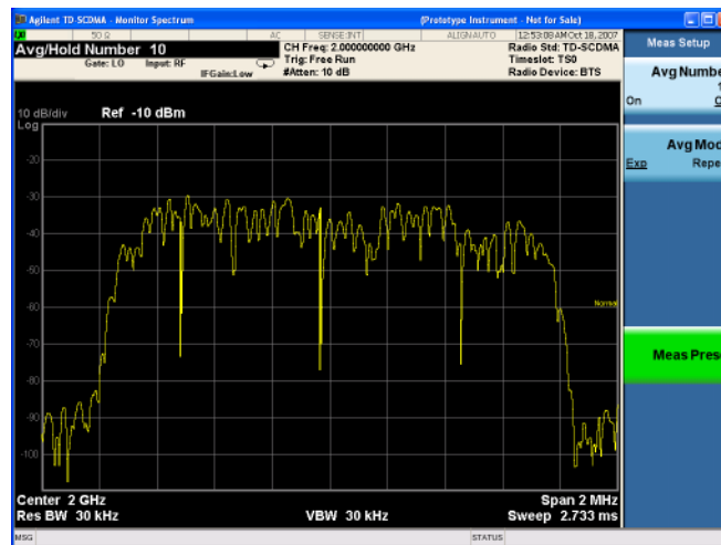
Monitor Spectrum Measurement
