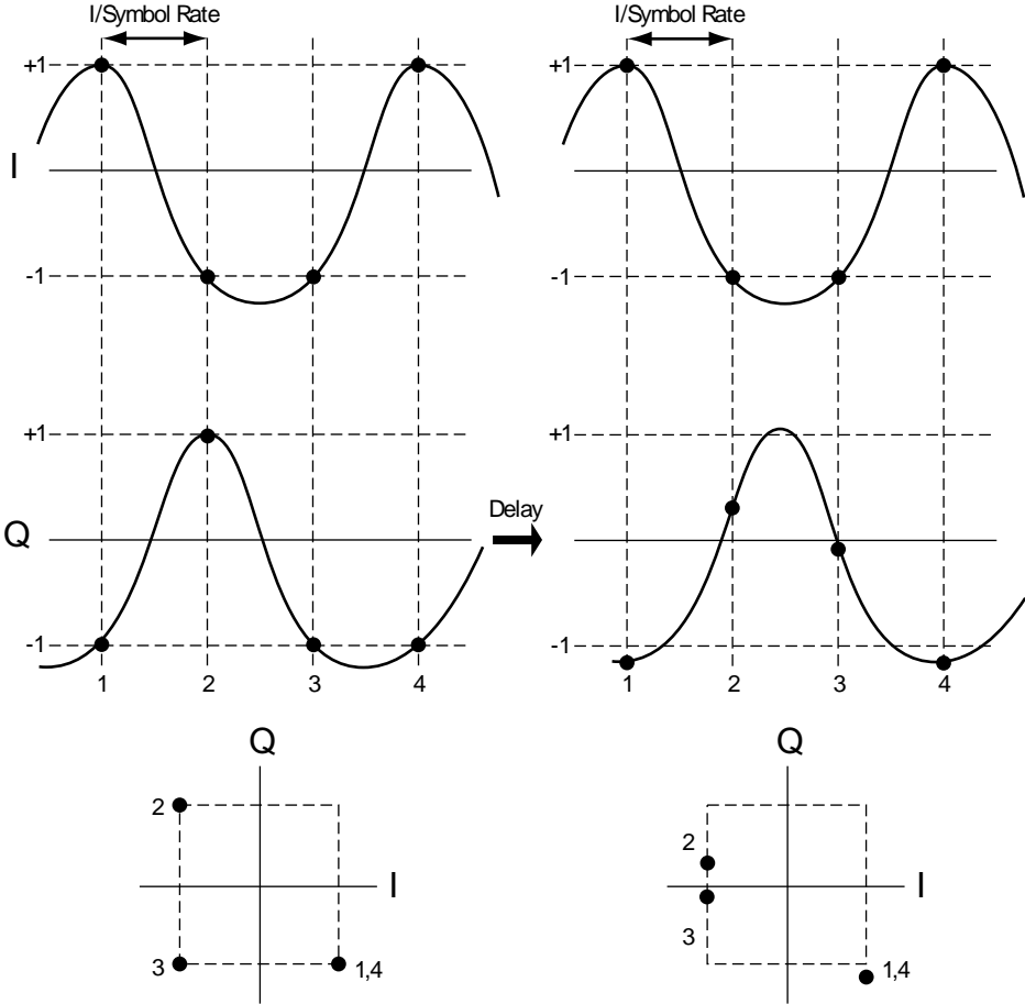
Figure 4-13 Delays in I/Q paths
