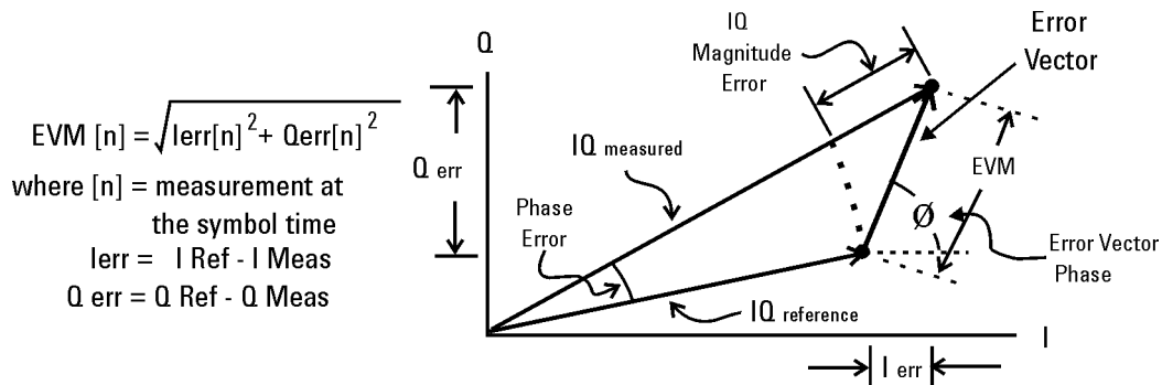
Figure 4-17 Error Vector Magnitude and Related Parameters
