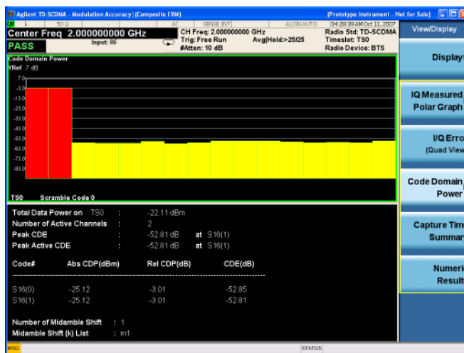
Figure 2-27 Modulation Accuracy - Code Domain Power View
