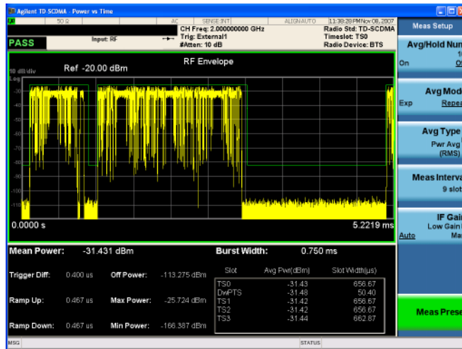
Figure 2-11 Power vs Time - Multi-Slot View (Meas Interval = 9)
