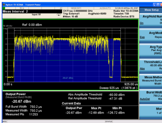
Figure 2-3 Transmit Power - Measured Burst Width
