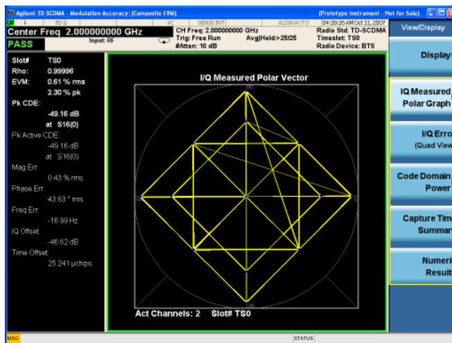
Figure 2-26 Modulation Accuracy - I/Q Measured Polar Graph View (Default)
