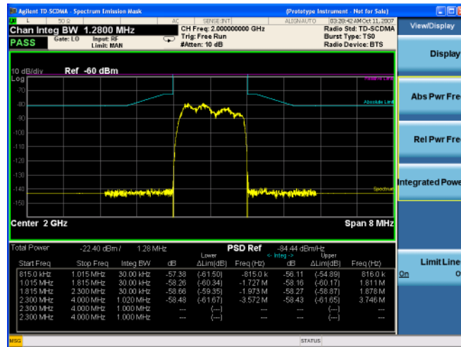
Figure 2-16 SEM - PSD Ref, Integrated Power view
