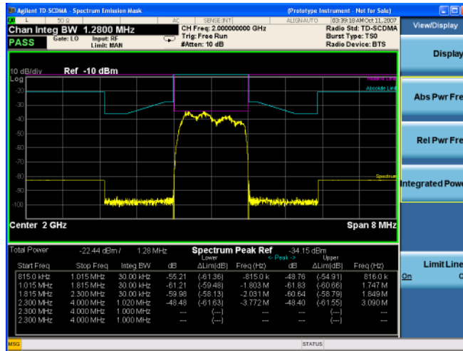
Figure 2-15 SEM - Spec Peak Ref, Rel Pwr Freq view
