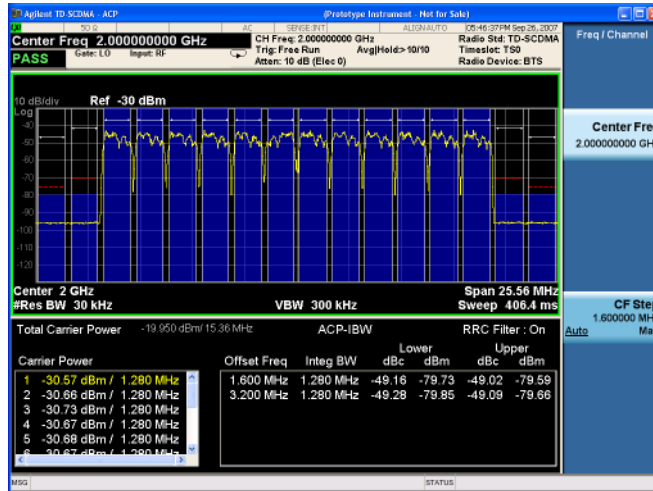
Figure 2-8 ACP - Multiple Carriers
