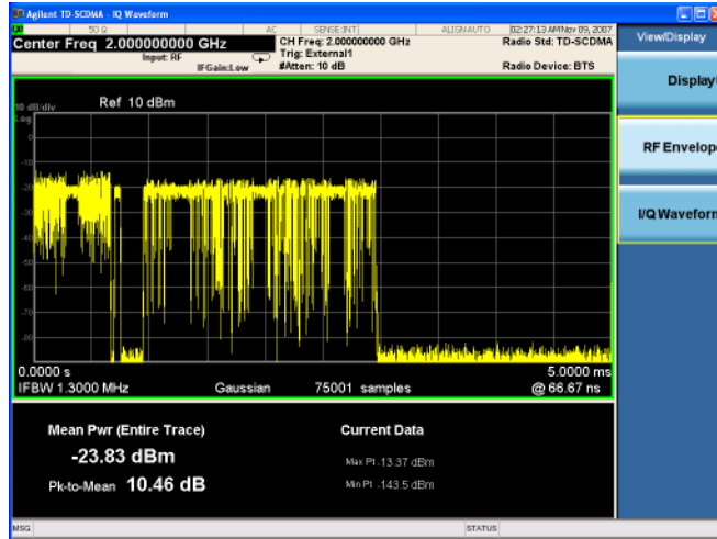
Figure 2-40 Monitor Spectrum Measurement - RF Envelope view (Default)
